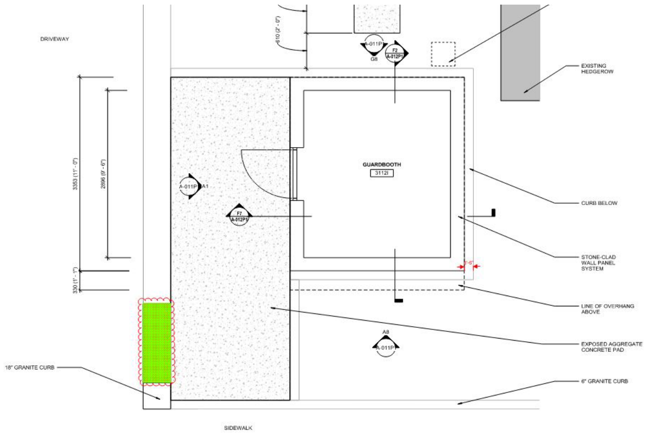
GUARDBOOTH - FLOOR PLAN - BELOW SILL - PHASE 1
